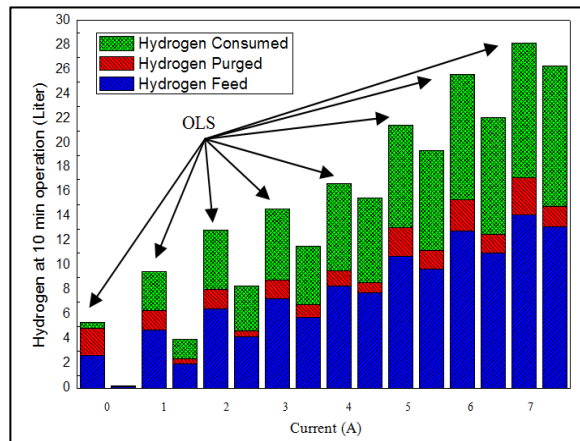
Figure 9. Total hydrogen consumption for OLS and CLS configuration
