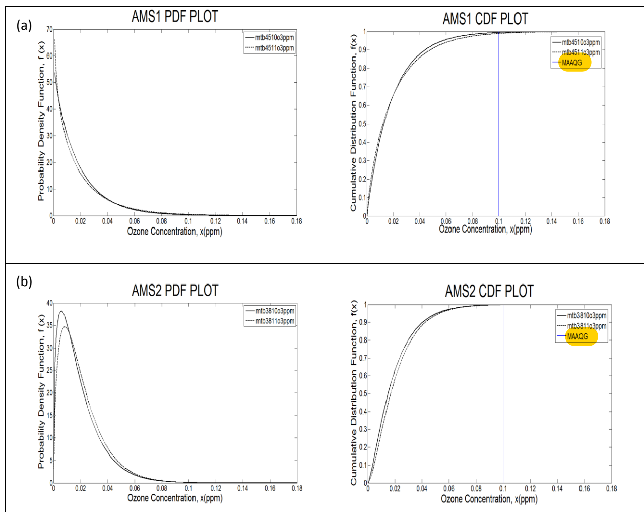
Figure 2. Gamma distribution PDF and CDF plots for both sites in 2010 and 2011 with MAAQG limit
