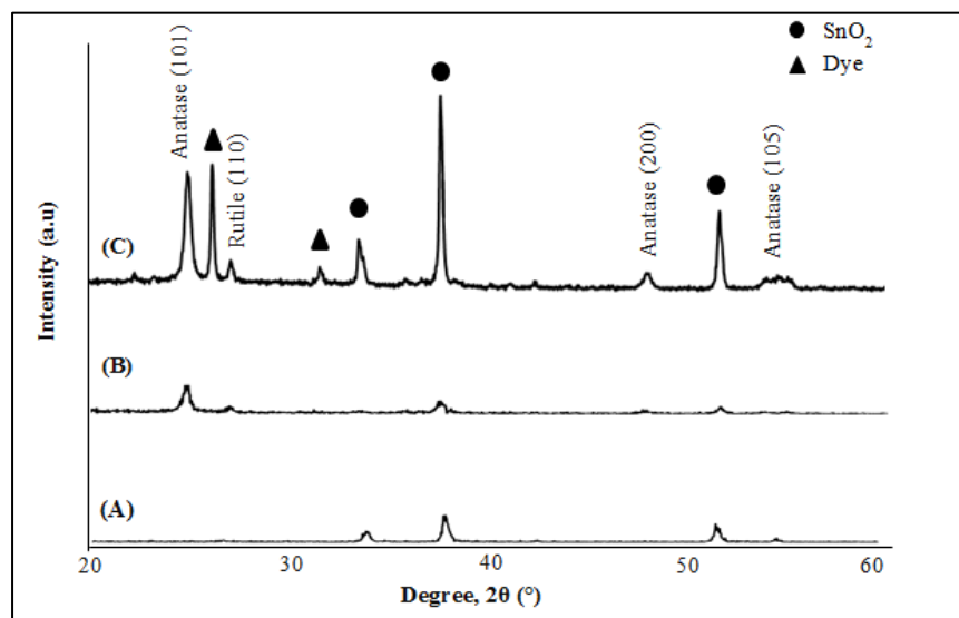
Figure 2. X-Ray Diffraction (XRD) pattern of (A) FTO, (B) \text{TiO}_2 and (C) dye-sensitized \text{TiO}_2 thin films deposited onto FTO
