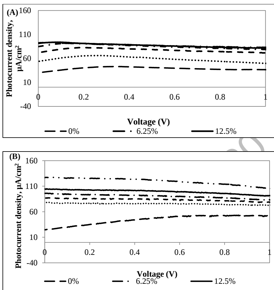
Figure 5. Performance of photocurrent density of (A) bare \text{TiO}_2 and (B) \text{TiO}_2 with dye sensitizer on different concentrations of pitaya peel dye in electrolyte
