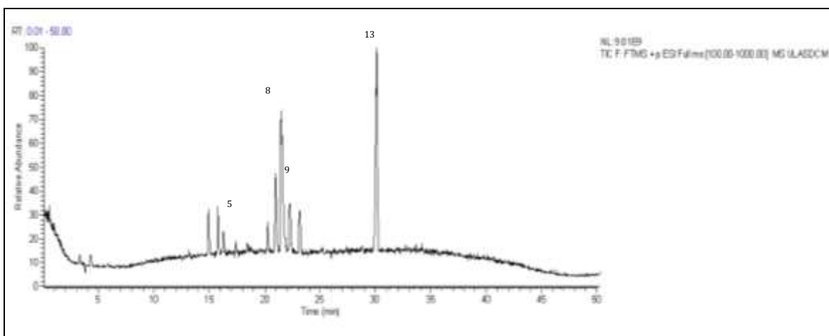
Figure 2. Chromatogram of DCM extract of U. lanosa ; the total ion current (TIC) in positive mode; numbers of identified peak are according to no. of reference compound shown in Table 1.
