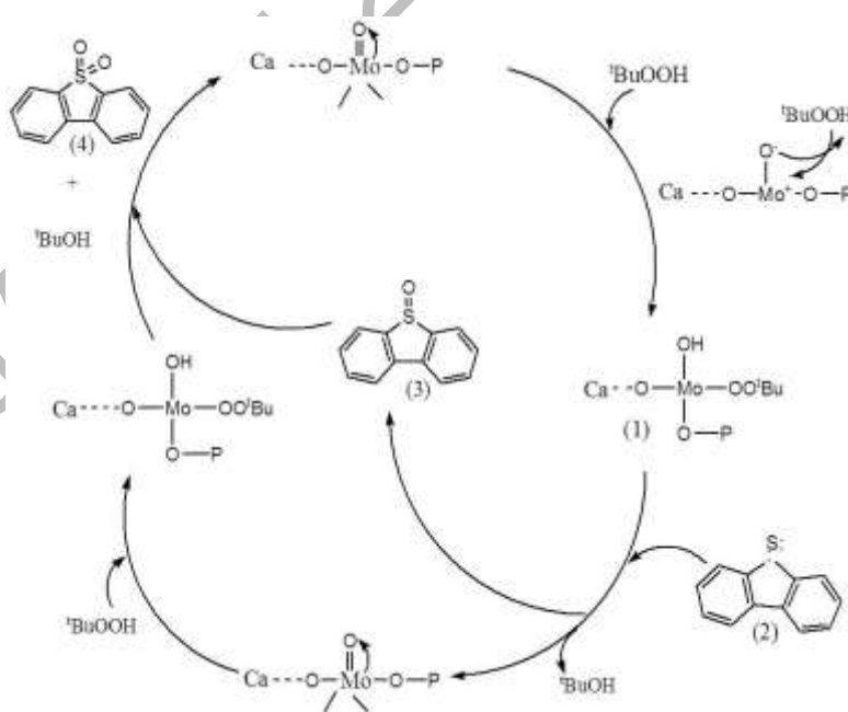
Figure 6. A proposed cyclic mechanism for the oxidation of dibenzothiophene by TBHP in the presence of \text{Ca}/\text{MoO}_3\text{-PO}_4/\text{Al}_2\text{O}_3 catalyst
