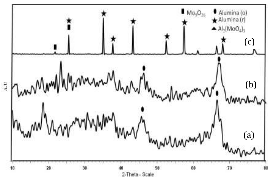
Figure 5. XRD diffractogram patterns of \text{Ca}/\text{MoO}_3\text{-PO}_4/\text{Al}_2\text{O}_3 calcined at (a) 500°C, (b) 700°C and (c) 900°C.
