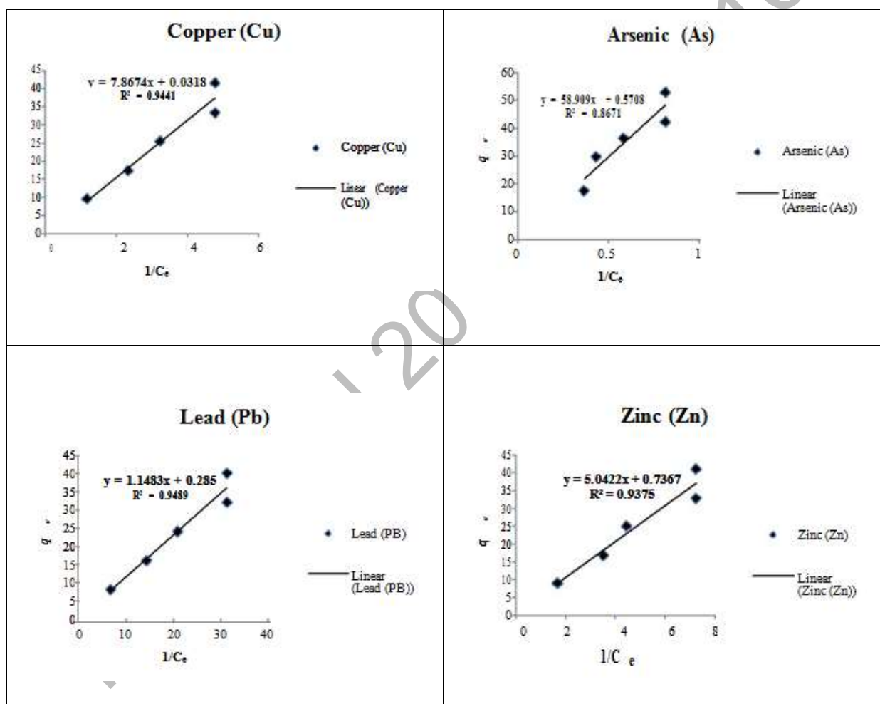
Figure 5. Plots of Langmuir isotherm for all heavy metals examined
