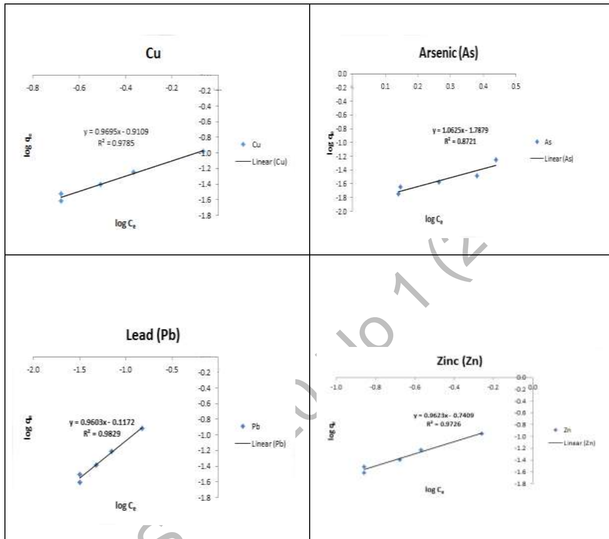
Figure 6. Plots of Freundlich isotherm for all heavy metals examined
