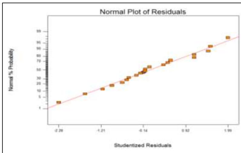
Figure 1. Normality plot of residuals
