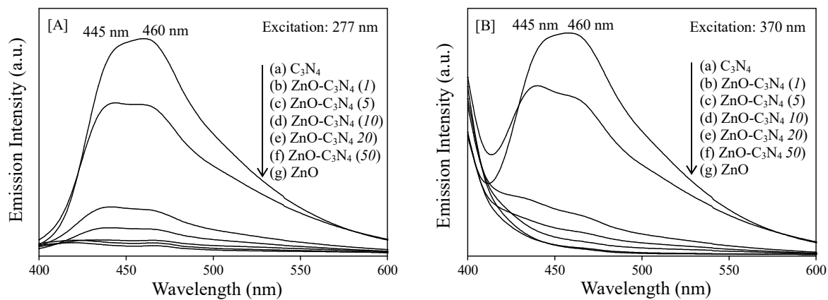
Figure 4 Emission spectra of (a) C_3N_4 , (b) ZnO-C_3N_4 (1), (c) ZnO-C_3N_4 (5), (d) ZnO-C_3N_4 (10), (e) ZnO-C_3N_4 (20), (f) ZnO-C_3N_4 (50) and (g) ZnO monitored at the excitation wavelength of [A] 277 and [B] 370 nm.
