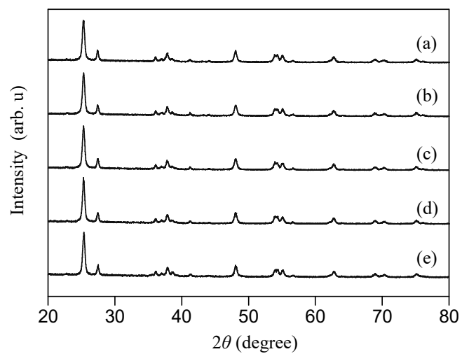
Figure 1 XRD patterns of (a) P25 \text{TiO}_2 , (b) 0.1 mol% Cu/P25 \text{TiO}_2 , (c) 0.5 mol% Cu/P25 \text{TiO}_2 , (d) 1 mol% Cu/P25 \text{TiO}_2 , and (e) 5 mol% Cu/P25 \text{TiO}_2 samples.
