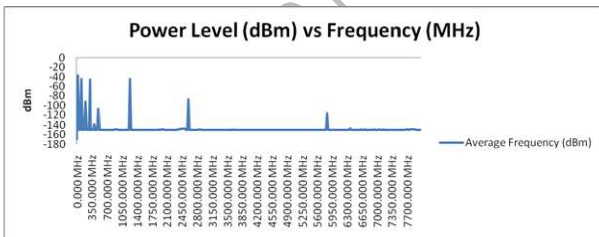
Figure 2. Graph of Power Level (dBm) vs Frequency (MHz) on 17 December 2014
