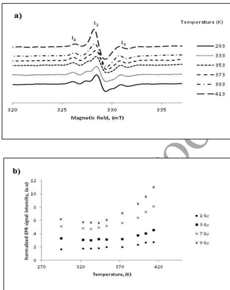
Figure 2. (a) The variation of EPR spectra recorded at different temperature for PT irradiated at a dose of 9 Gy. (b) The EPR signal intensity of PT sample ( I_2 ) irradiated at 1, 3, 7 and 9 Gy recorded at different temperature.
