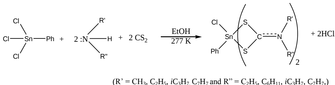
Figure 1. General reaction between secondary amine, carbon disulphide and phenyltin(IV) trichloride.
