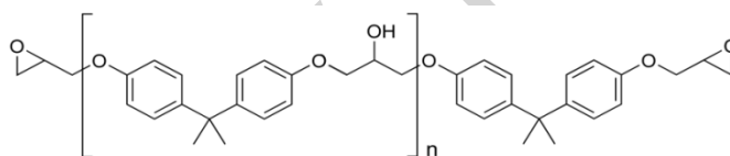
Figure 1. Chemical structures of PDGEBA.
