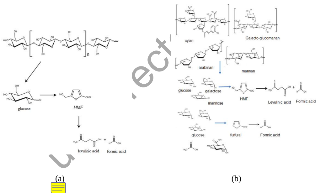
Figure 1. (a) Cellulose and (b) hemicellulose pathways for bioconversion [9]
