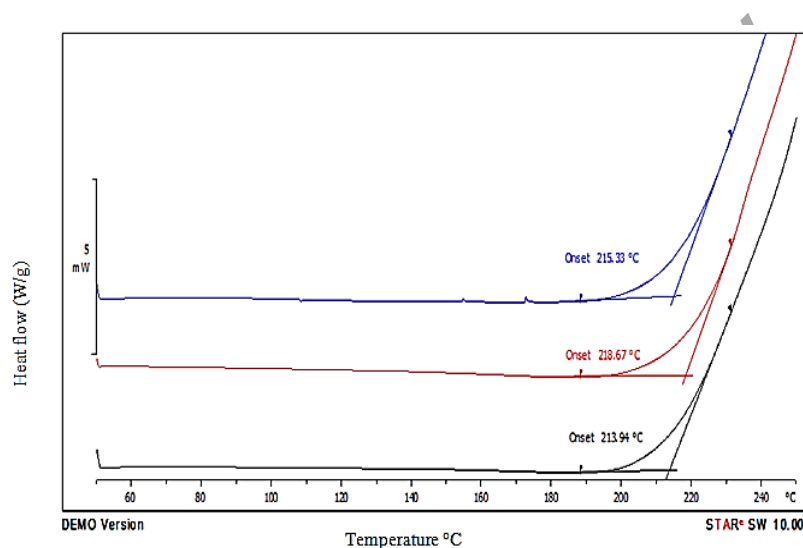
Figure 6. The PDSC exotherm curves of D2EBD as (OT).
