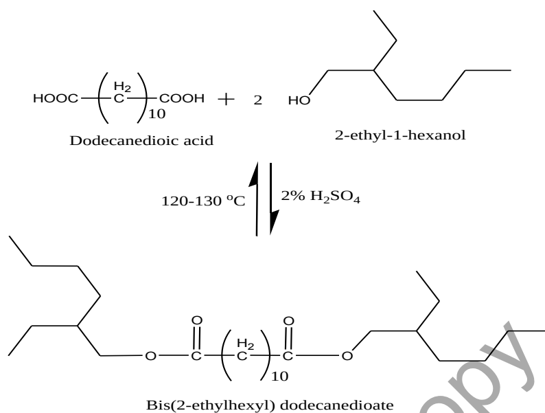
Figure 1. The reaction process of dicarboxylic acids and 2-ethyl-1-hexanol to form D2EHD.
