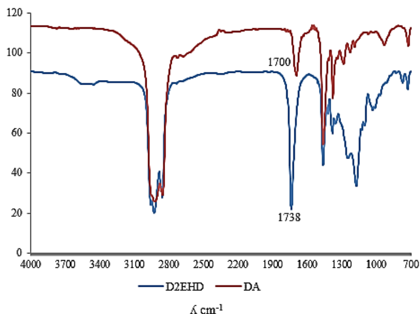
Figure 4. Comparison FTIR spectrum of D2EHD and DA
