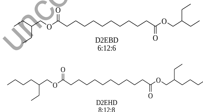
Figure 5. Chemical structure of D2EHD and D2EBD
