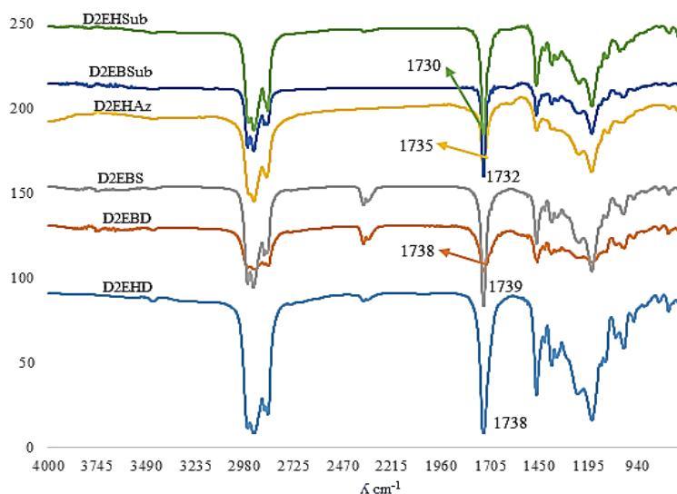
Figure 3. FTIR spectrum synthesized dicarboxylate ester
