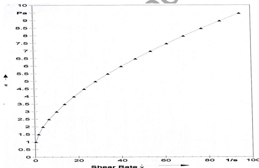
Figure 7. Shear stress vs. shear rate plots of D2EHD at 25 °C
