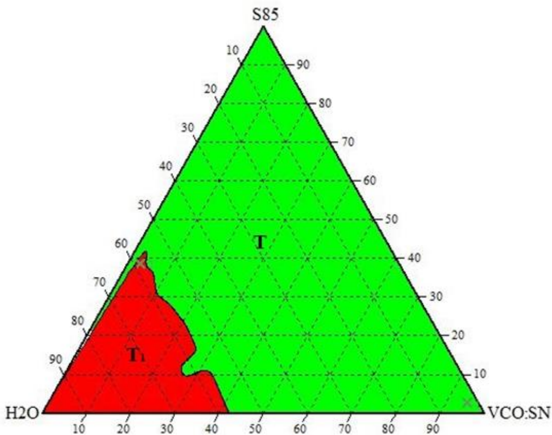
Figure 5. Ternary Phase Diagram of Span 85/VCO:Swiftlet Nest/Water.(T – Two phase region; T_1 – Three phase region)
