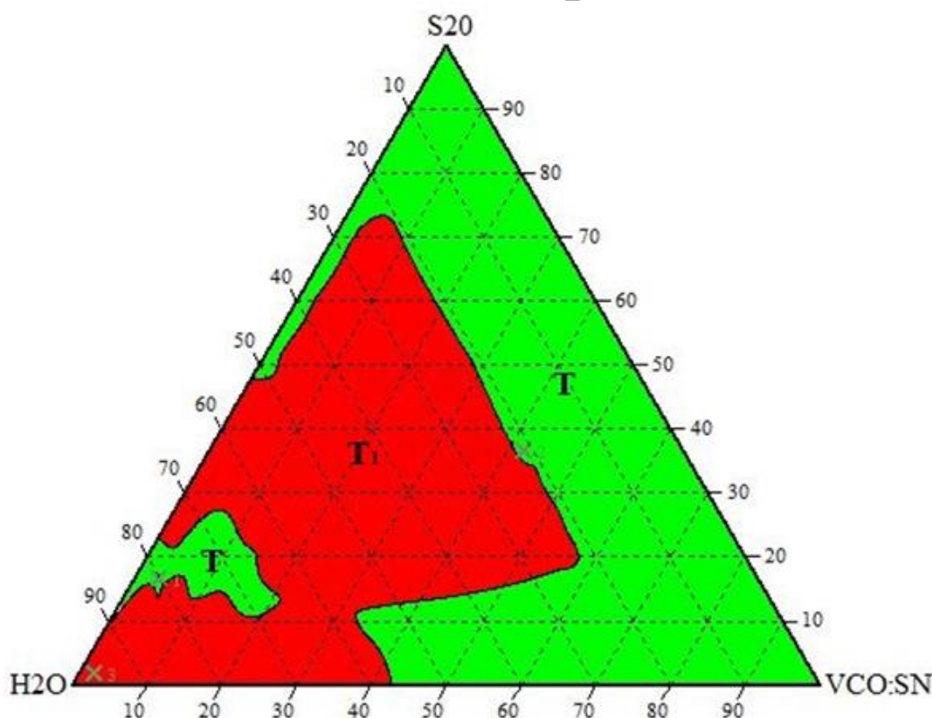
Figure 3. Ternary Phase Diagram of Span 20/VCO:Swiftlet Nest/Water(T – Two phase region; T_1 – Three phase region)
