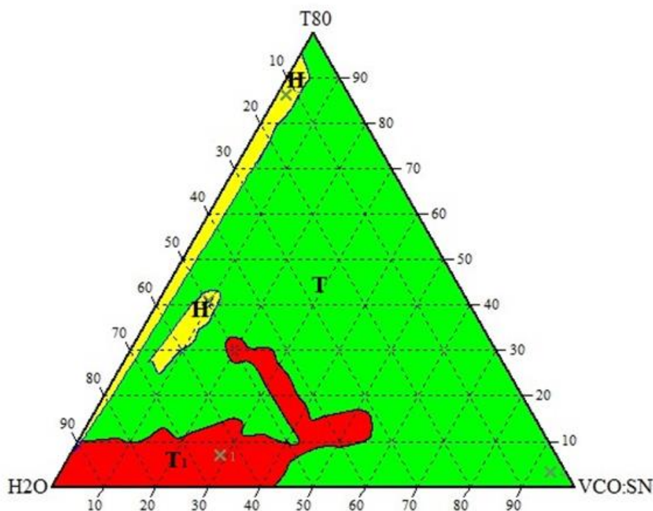
Figure 1. Ternary Phase Diagram of Tween 80/VCO:Swiftlet Nest/Water. (H – Homogenous region; T – Two phase region; T_1 – Three phase region)
