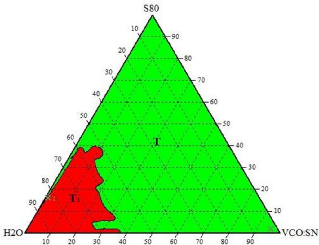
Figure 4. Ternary Phase Diagram of Span 80/VCO:Swiftlet Nest/Water.(T – Two phase region; T_1 – Three phase region)
