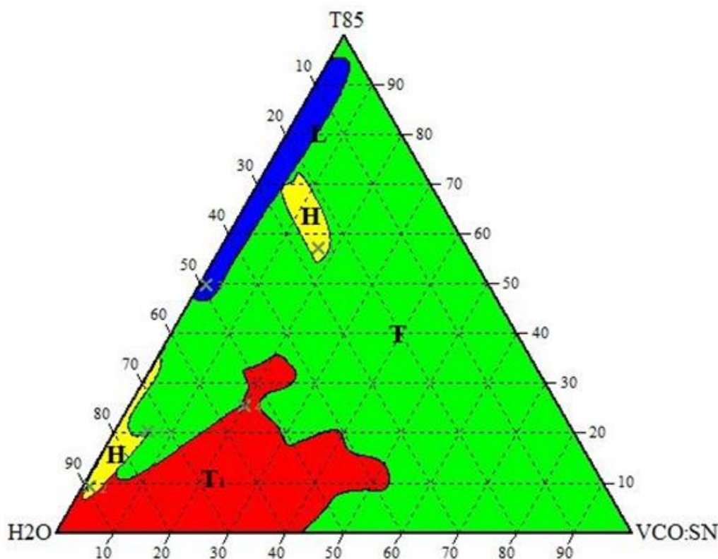
Figure 2. Ternary Phase Diagram of Tween 85/VCO:Swiftlet Nest/Water. (H – Homogenous region; L – Isotropic region; T – Two phase region; T 1 – Three phase region)
