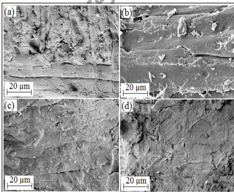
Figure 1. FESEM images of untreated lignocellulosic biomasses (a) kempas, (b) jelutong, (c) kenaf, (d) rice husk
