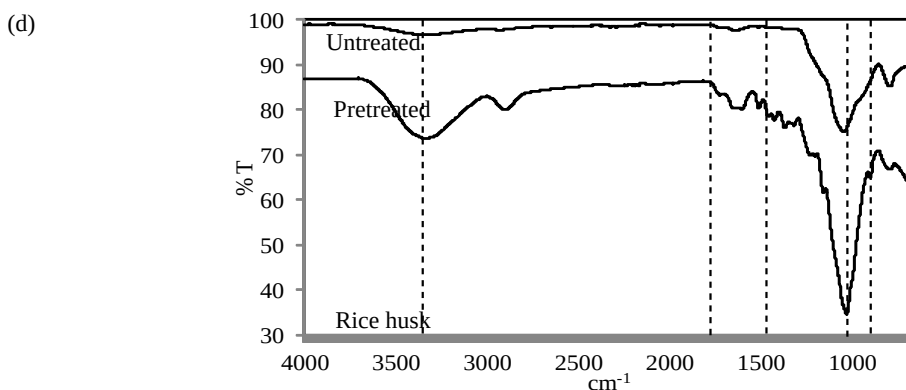
Figure 3. ATR FT-IR spectral analyses of untreated and pretreated lignocellulosic biomasses. FT-IR spectral bands ( \text{cm}^{-1} ): (1)= 3338; (2)= 1732; (3)= 1457; (4)= 1048; (5) 895
