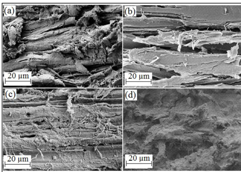
Figure 2. FESEM images of pretreated lignocellulosic biomasses (a) kempas, (b) jelutong, (c) kenaf, (d) rice husk
