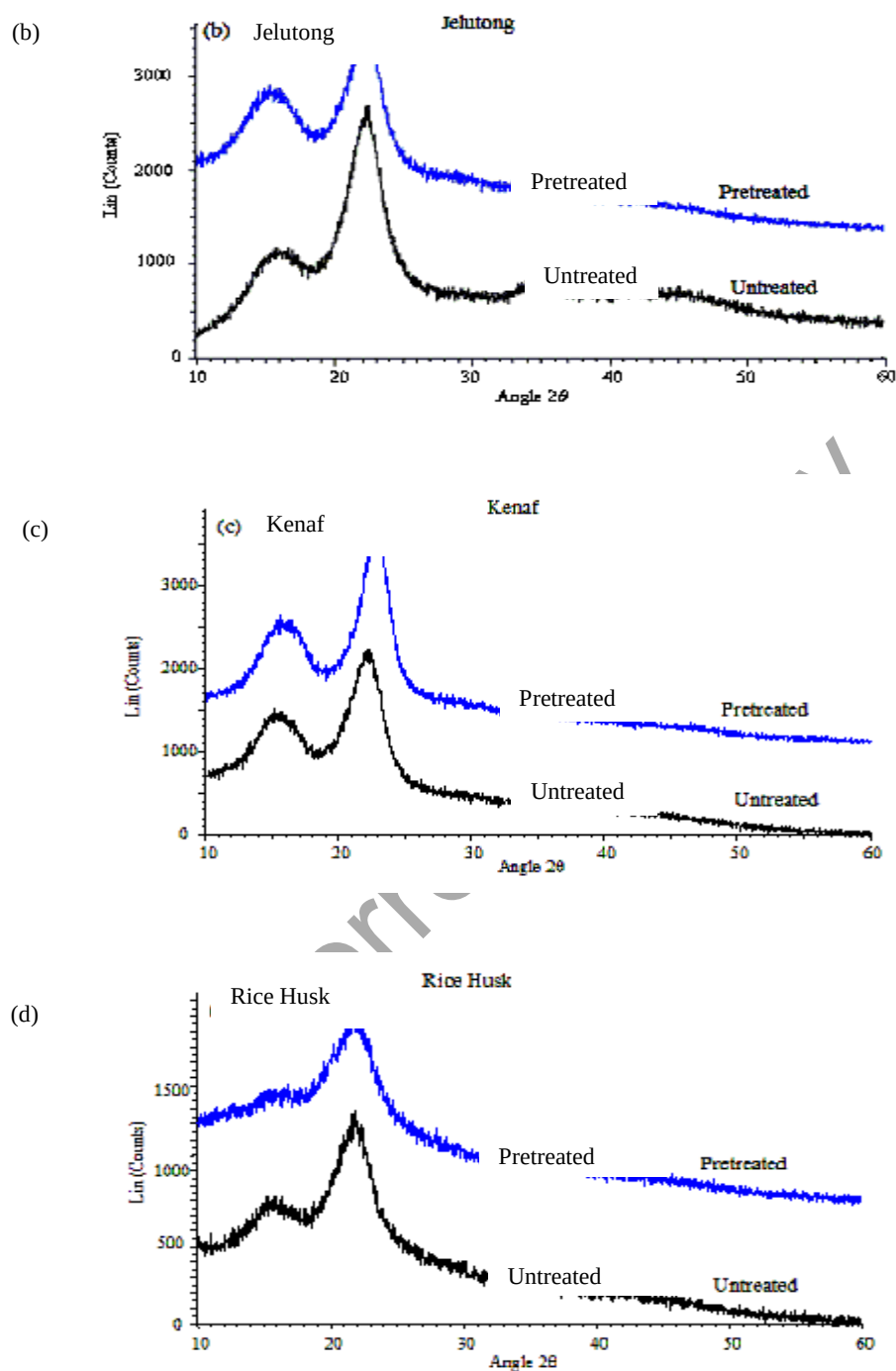
Figure 4. XRD analyses of untreated and pretreated biomasses
