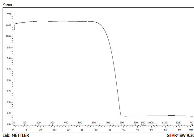
Figure 1. TGA curve of raw seashell
