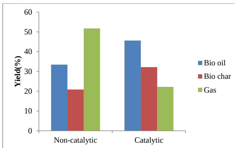
Figure 3. The product yield at 550 °C in non-catalytic and catalytic pyrolysis of biomass
