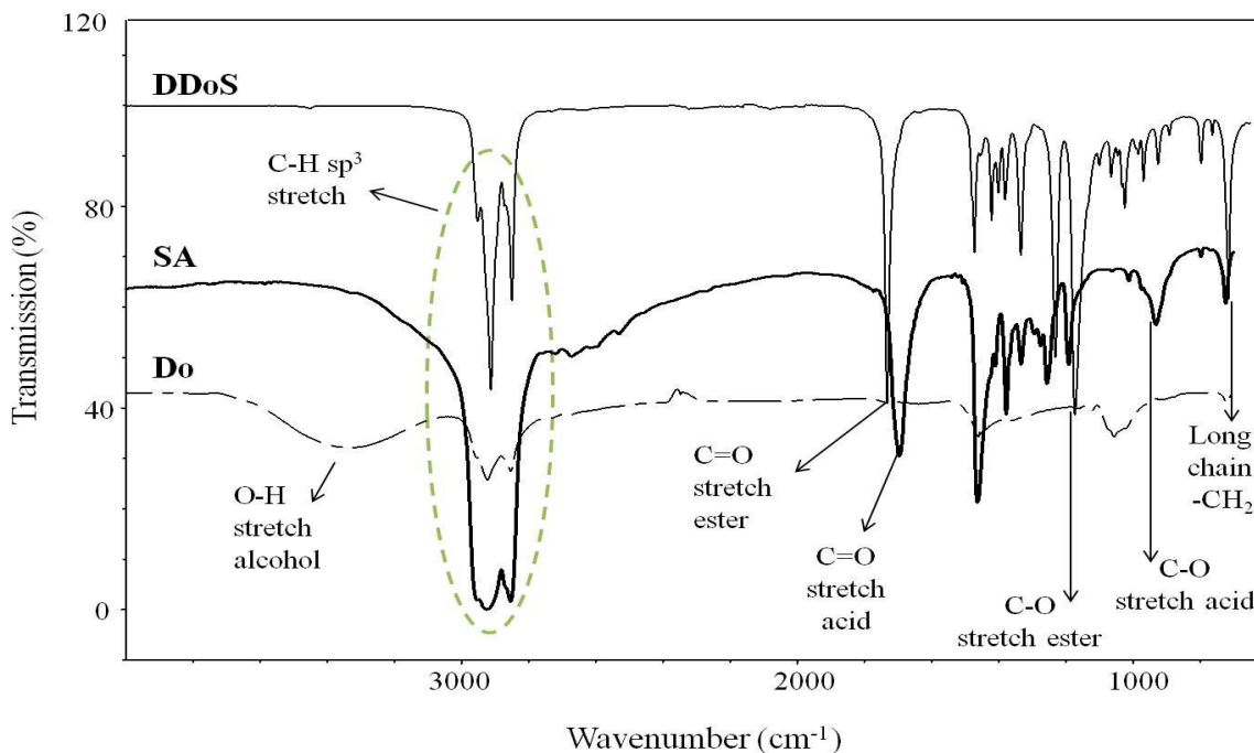
Figure 2. Comparison of FTIR spectra for 1,8-didodecanyl suberate (DDoS), suberic acid (SA) and 1-dodecanol (Do)
