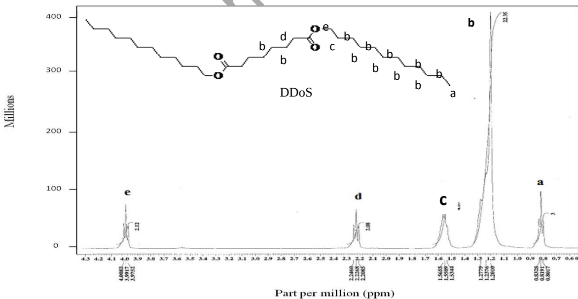
Figure 3. 1 H NMR spectrum for 1,8-didodecanyl suberate (DDoS)
