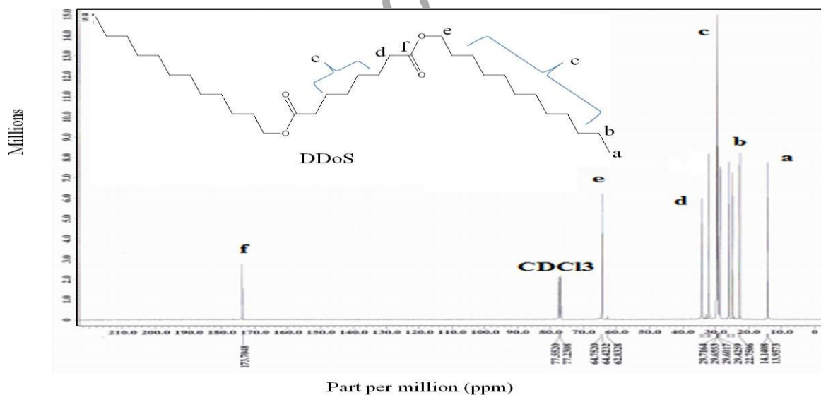
Figure 4. ^{13}\text{C} NMR spectrum of 1,8-didodecanyl suberate (DDoS).
