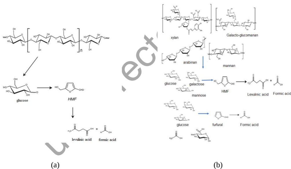
Figure 1. (a) Cellulose and (b) hemicellulose pathways for bioconversion [9]
