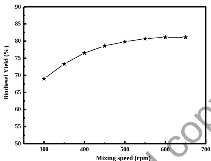
Figure 7. Effect of agitator speed on biodiesel yield (%) in the presence of Mo/ \gamma -Al 2 O 3 -20 wt% CeO 2 catalyst at methanol/oil molar ratio of 30:1, reaction temperature of 110 °C, reaction time of 270 min and catalyst loading of 7 wt%.
