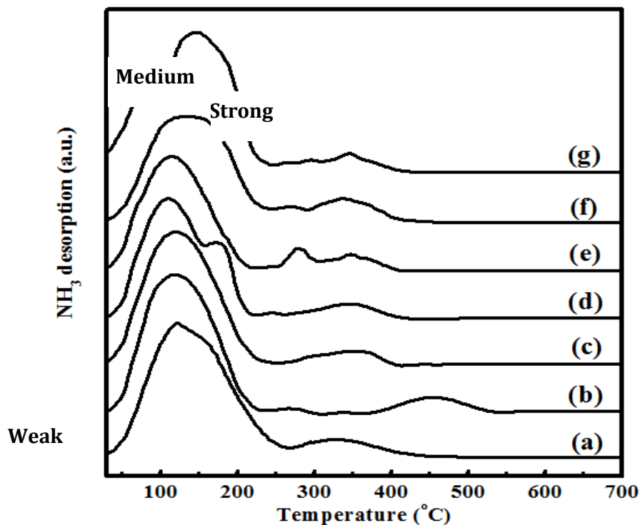
Figure 3. \text{NH}_3 -TPD patterns of (a) \text{CeO}_2 (b) \gamma\text{-Al}_2\text{O}_3 (c) \text{Mo}/\gamma\text{-Al}_2\text{O}_3 (d) \text{Mo}/\gamma\text{-Al}_2\text{O}_3 -5 wt% \text{CeO}_2 (e) \text{Mo}/\gamma\text{-Al}_2\text{O}_3 -10 wt% \text{CeO}_2 (f) \text{Mo}/\gamma\text{-Al}_2\text{O}_3 -15 wt% \text{CeO}_2 (g) \text{Mo}/\gamma\text{-Al}_2\text{O}_3 -20 wt% \text{CeO}_2 catalysts.
