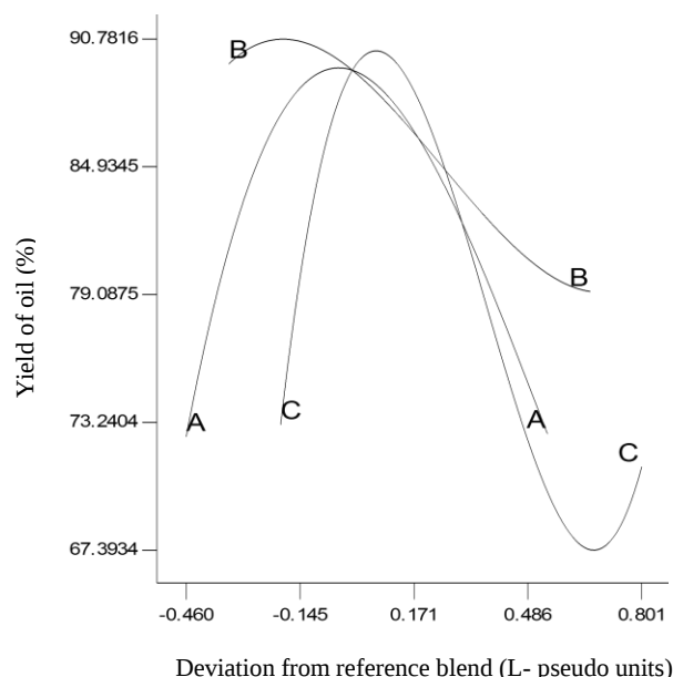
Figure 5. Trace Plot (Piepel) for oil yield % as a function of component mix of three enzymes (A: CTe2, B: HTec2, C: Pectinex) in reference to the optimum enzyme mixture
