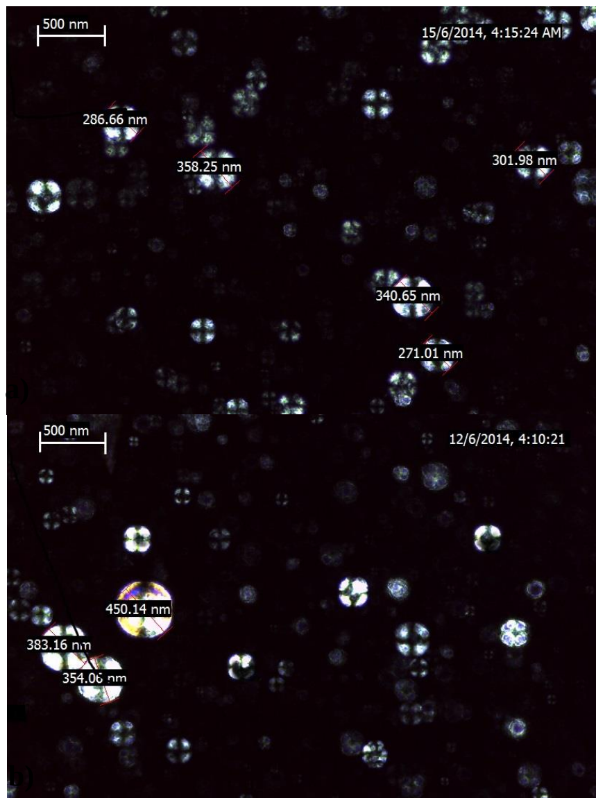
Figure 1. Polarized light microscope images of a) Amino Acid based Vesicles (AABV) and b) Amino Acid based Vesicles carrying Radiosensitizer (AABVRS) indicating vesicle formation through X cross formation
