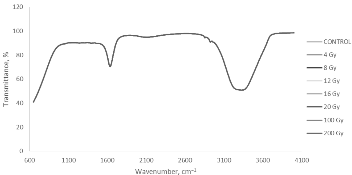
Figure 4. FTIR spectra of Amino Acid based Vesicles carrying Radiosensitizer (AABVRS) after being irradiated at 0 Gy, 4 Gy, 8 Gy, 12 Gy, 16 Gy, 20 Gy, 100 Gy and 200 Gy.
