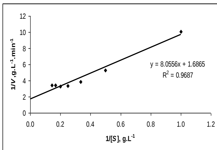
Figure 4. Lineweaver-Burk plot
