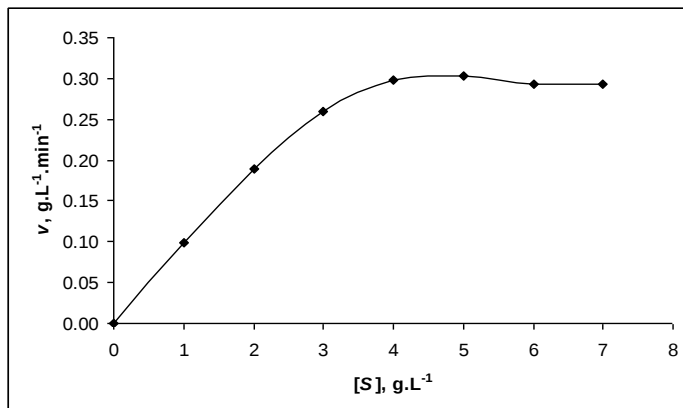
Figure 3. Michaelis-Menten plot
