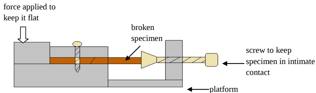
Figure 2. Schematic of the healing platform for the fractured Izod impact specimens
