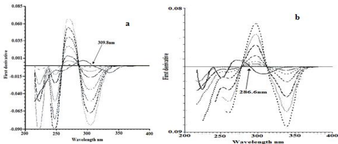
Figure 5. (a) First derivative absorption spectra of 10 µg/mL of LMT ( — ) and (1.0-50.0) µg/mL of CBZ (.....), (b) 6.0 µg/mL of CBZ ( — ) and (1.0-80.0) µg/mL of LMT ( ..... ) using ethanol: water (2:1) as a blank (smoothing = 3.0 nm).
