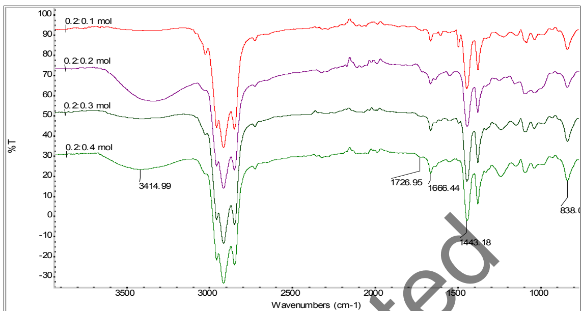
Figure 7. IR spectra of LNRs prepared at various concentration of sodium nitrite and 0.2 mol hydrogen peroxide
