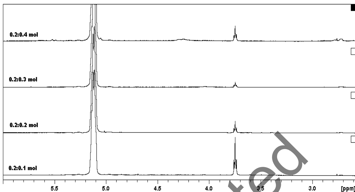
Figure 2. ^1\text{H} NMR spectra of LNRs prepared at 0.2 mol of hydrogen peroxide and various concentration of sodium nitrite
