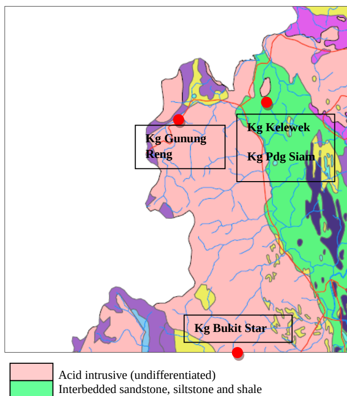
Figure 1: The geological map of the sampling area
