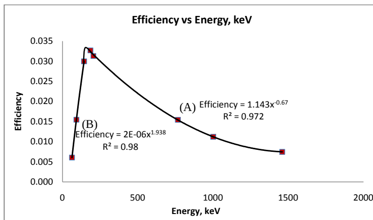
Figure 2: Efficiency Calibration using \text{UO}_3 and KCl by Gamma Spectrometry
