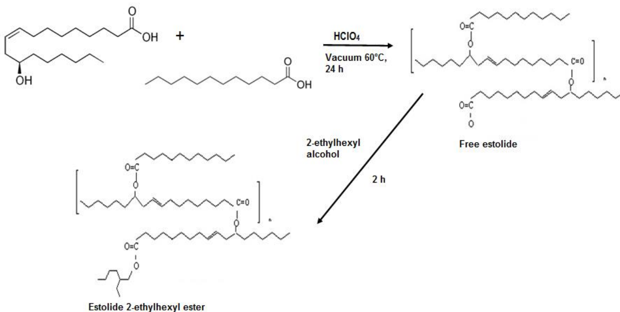
Figure 1: Synthesis of estolide 2-ethylhexyl ester
