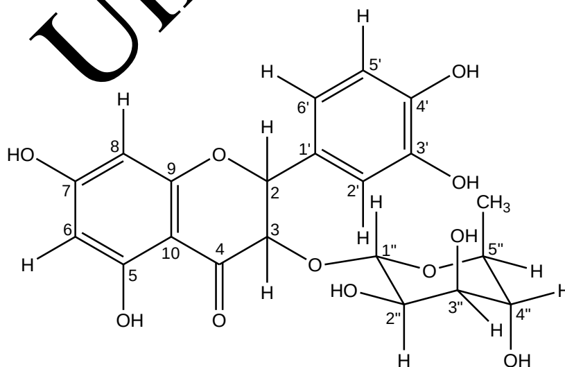
Figure 3. Astilbin
