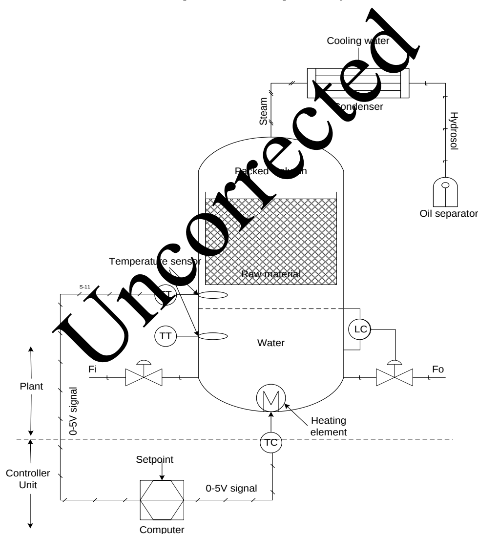
Figure 1. Steam Distillation Process for Essential Oil Extraction
