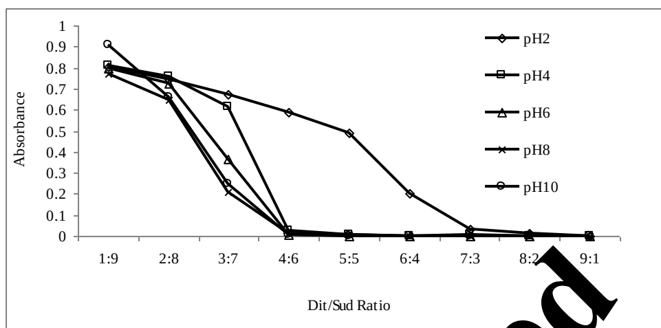
Figure 3c. Effect of the pH on the reduction of dye in 0.3% sodium dithionite.
