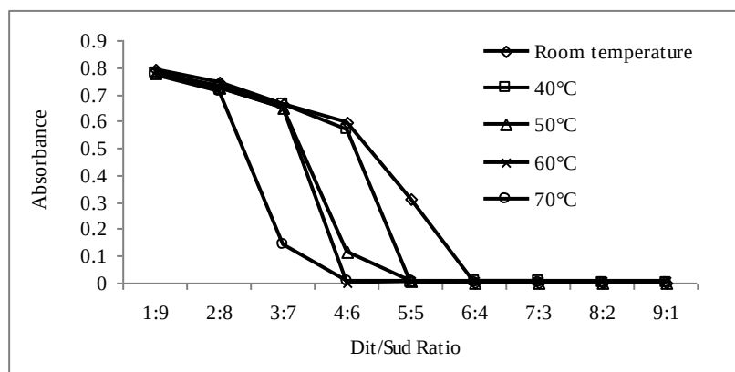
Figure 2b. Effect of temperature on the reduction of dye in 0.25% sodium dithionite.
